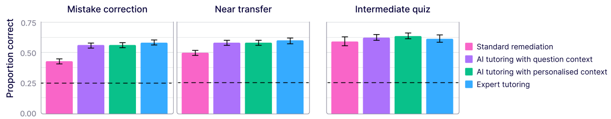
Figure 4 | One-to-one tutoring improved student performance across proximate and intermediate learning measures. (left, centre) For proximate in-platform outcomes, expert tutoring and both forms of AI tutoring promoted similar levels of mistake correction and near transfer. Students in all three tutoring conditions substantially outperformed students receiving standard remediation. (right) On the intermediate curriculum quiz, tutored students continued to score higher than students receiving standard remediation. Bar height and error bars indicate posterior estimates and 95% credible intervals, whereas dashed lines represent random chance.
