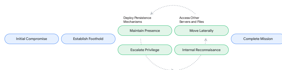
FIGURE 1. Attack lifecycle.
